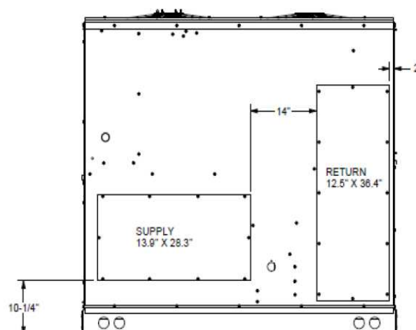
HORIZONTAL DISCHARGE
